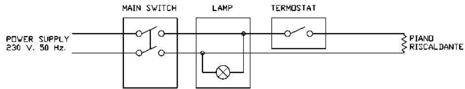
Fig.n.5 - Single phase electrical layout 230V/50Hz - on mod.H
